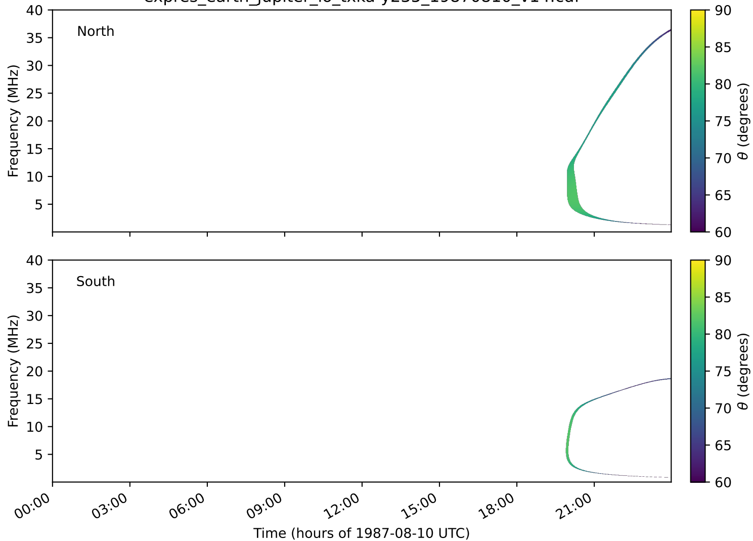
expres_earth_jupiter_io_txka-y235_19870810_v14.cdf
