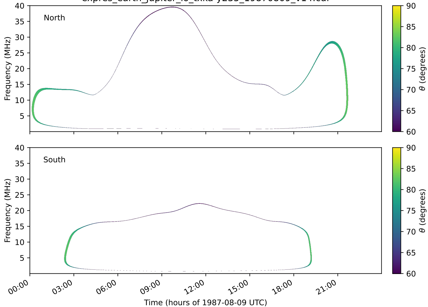
expres_earth_jupiter_io_txka-y235_19870809_v14.cdf
