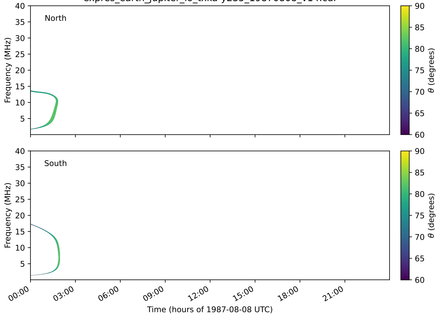
expres_earth_jupiter_io_txka-y235_19870808_v14.cdf
