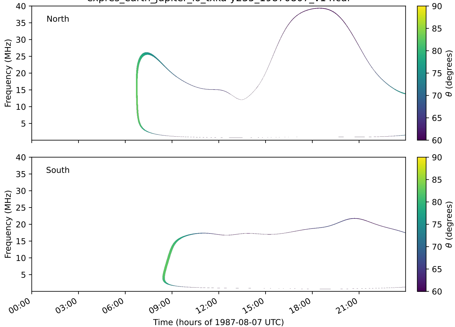
expres_earth_jupiter_io_txka-y235_19870807_v14.cdf
