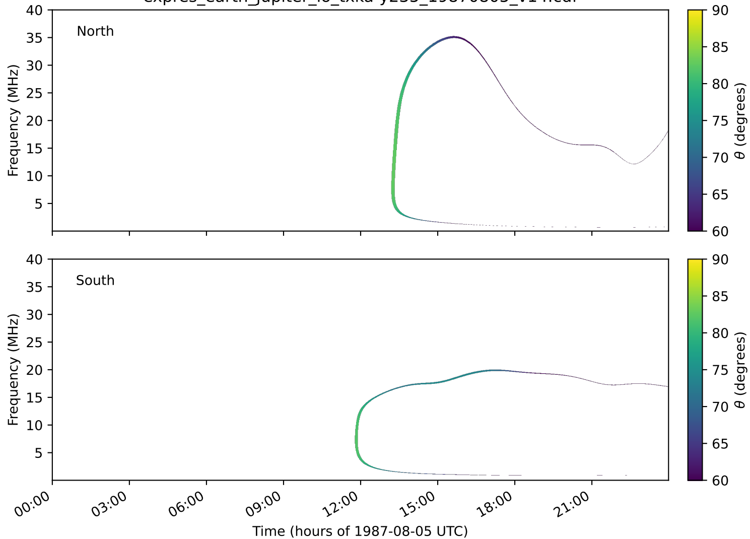
expres_earth_jupiter_io_txka-y235_19870805_v14.cdf
