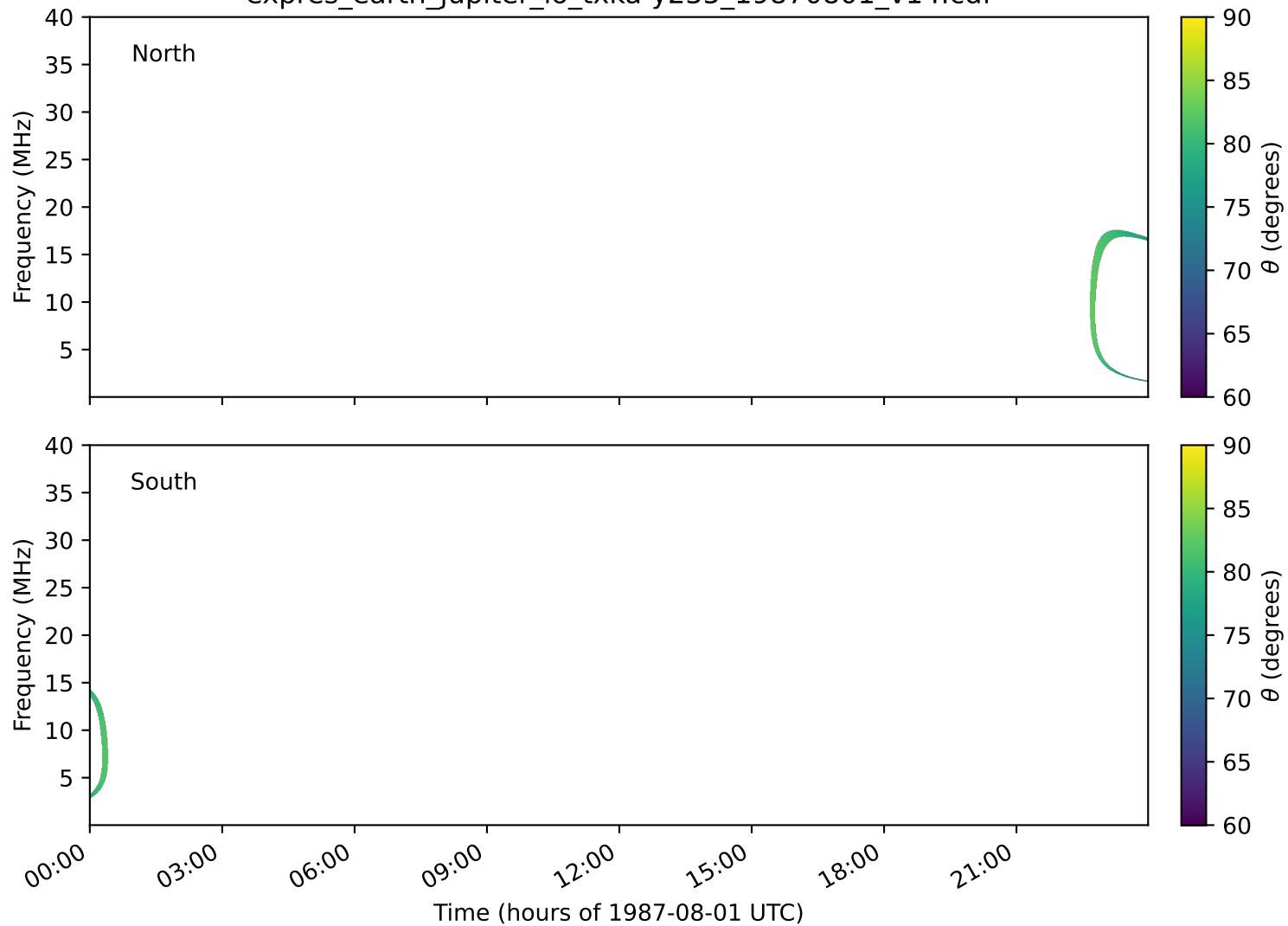
expres_earth_jupiter_io_txka-y235_19870801_v14.cdf
