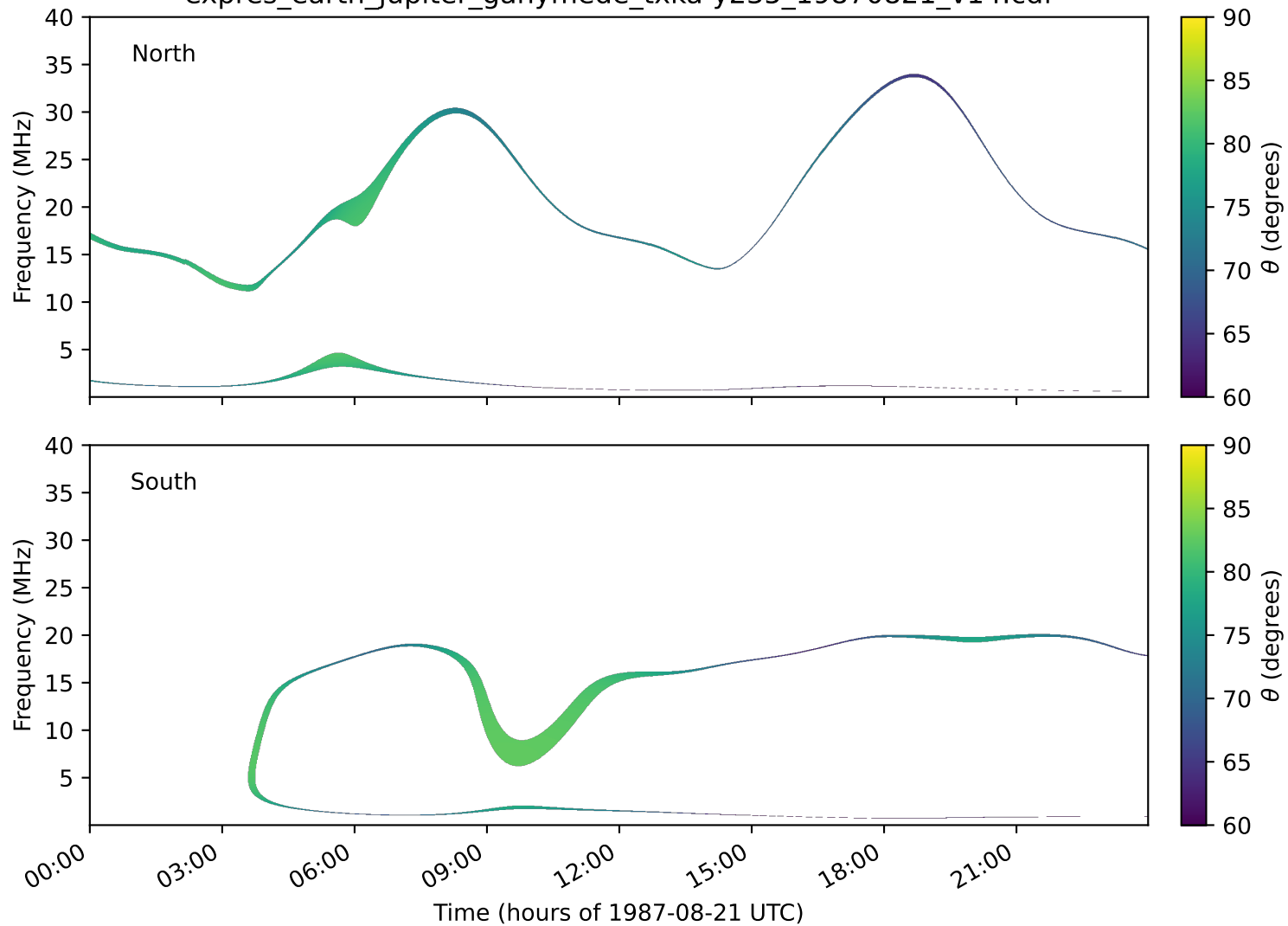
expres_earth_jupiter_ganymede_txka-y235_19870821_v14.cdf
