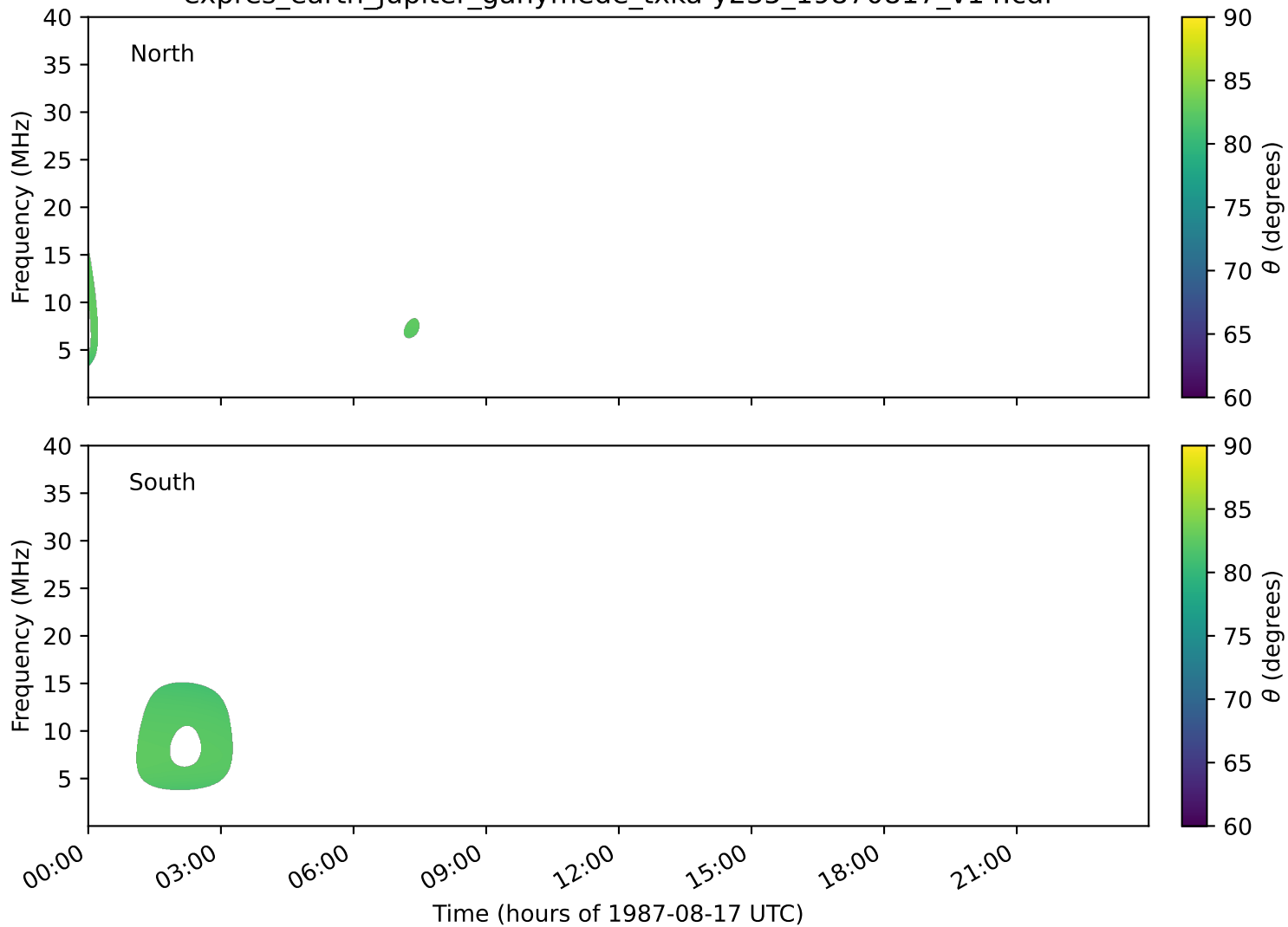
expres_earth_jupiter_ganymede_txka-y235_19870817_v14.cdf
