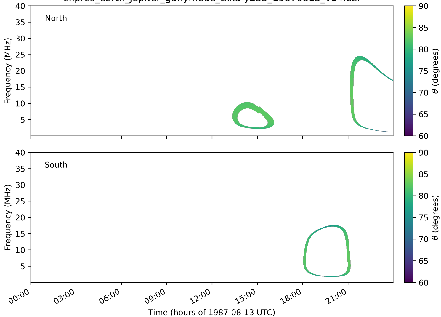
expres_earth_jupiter_ganymede_txka-y235_19870813_v14.cdf
