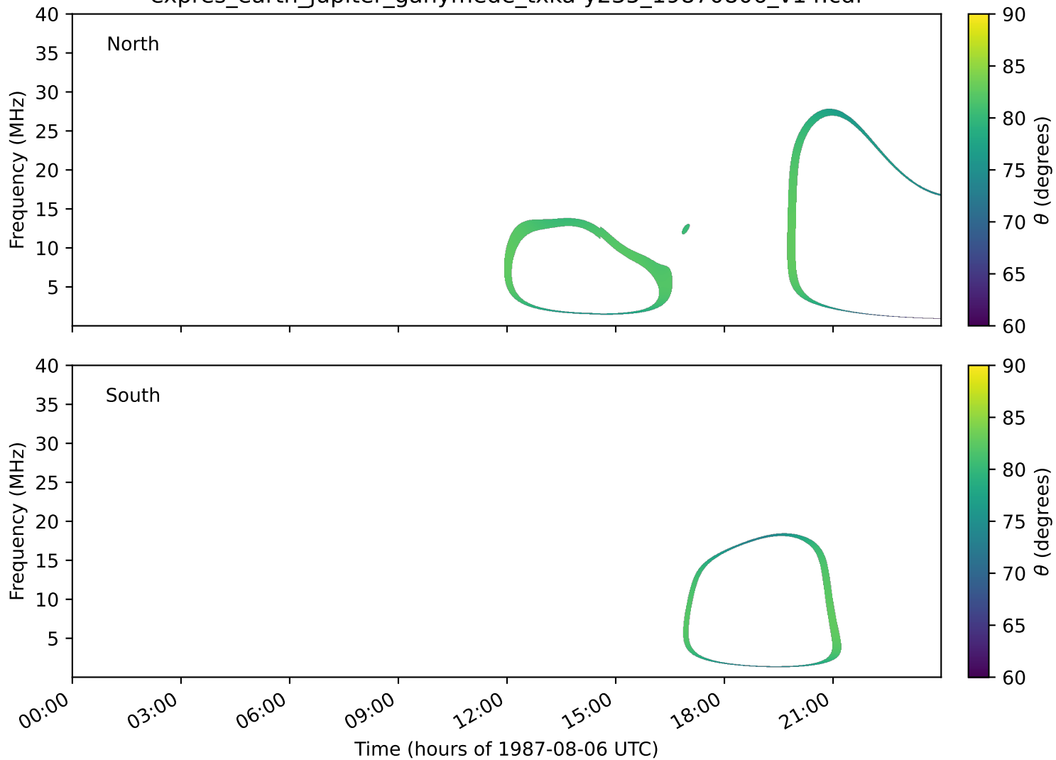
expres_earth_jupiter_ganymede_txka-y235_19870806_v14.cdf
