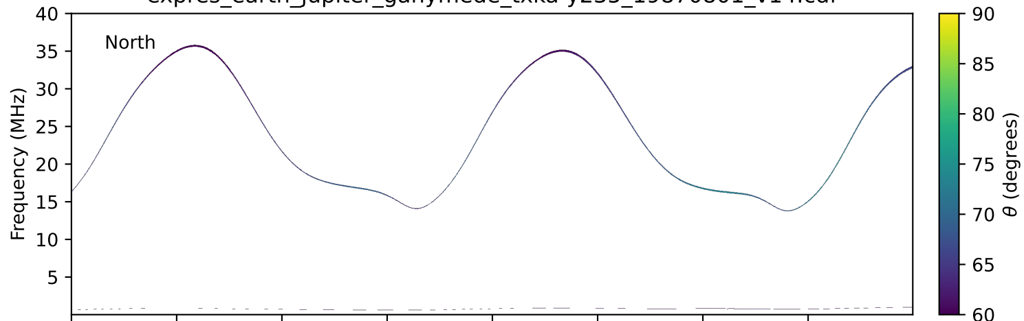
expres_earth_jupiter_ganymede_txka-y235_19870801_v14.cdf
