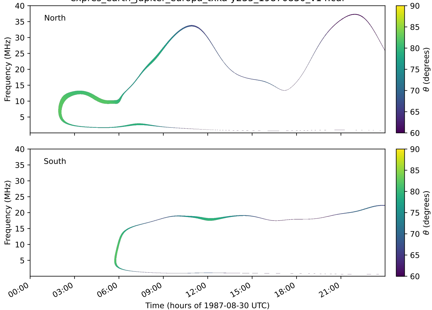
expres_earth_jupiter_europa_txka-y235_19870830_v14.cdf
