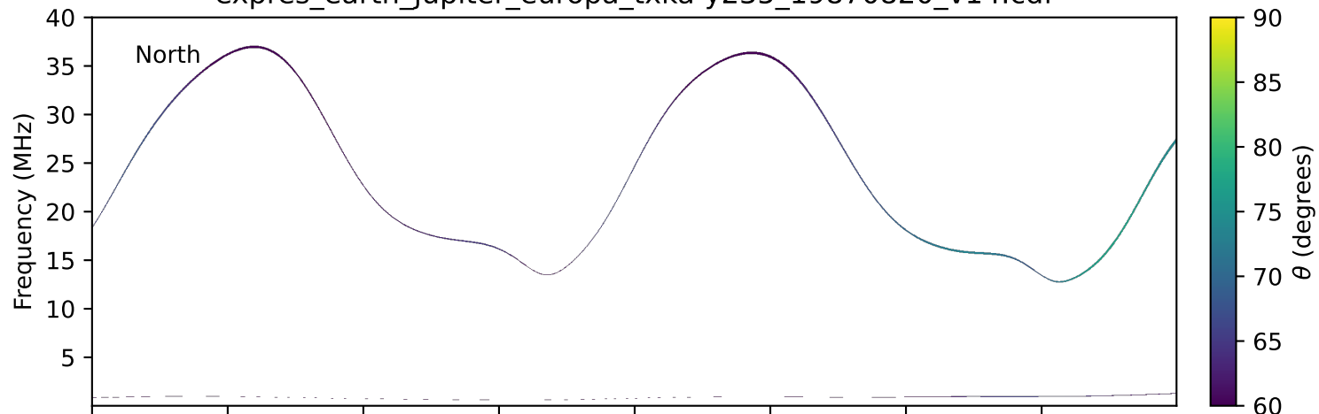
expres_earth_jupiter_europa_txka-y235_19870820_v14.cdf
