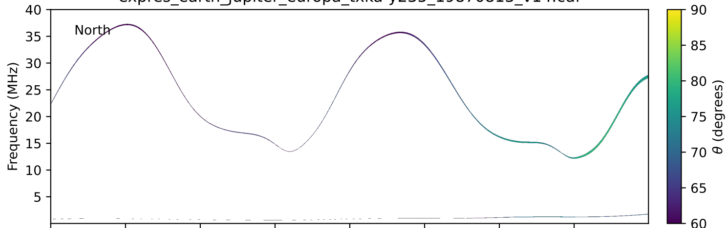
expres_earth_jupiter_europa_txka-y235_19870813_v14.cdf
