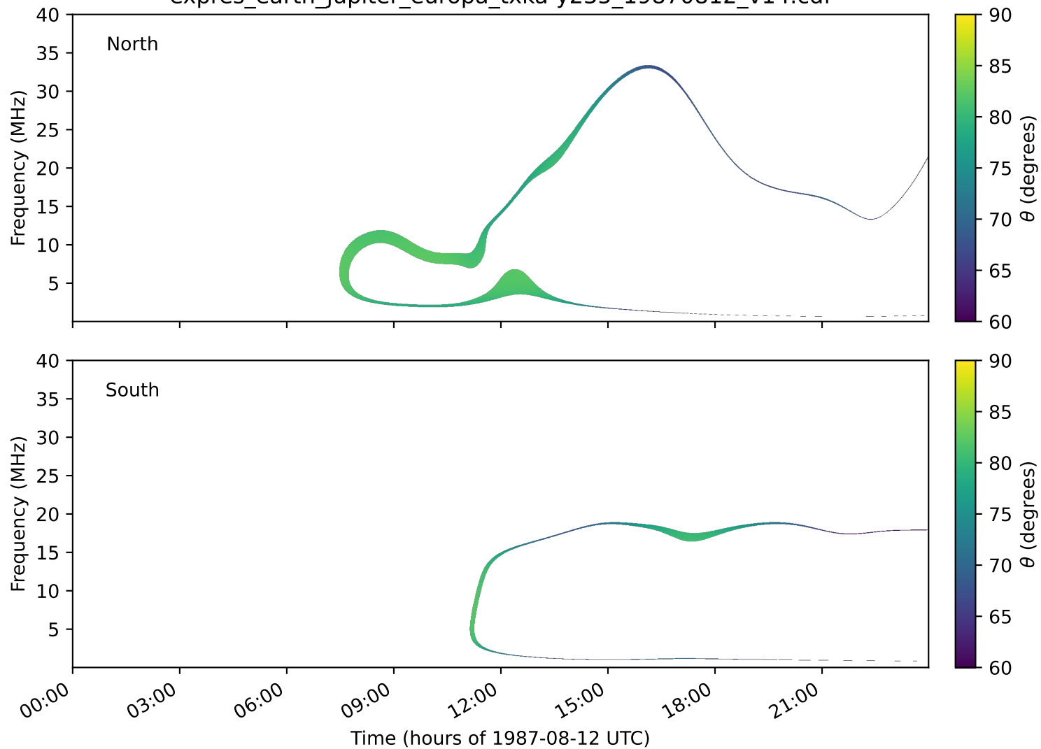
expres_earth_jupiter_europa_txka-y235_19870812_v14.cdf
