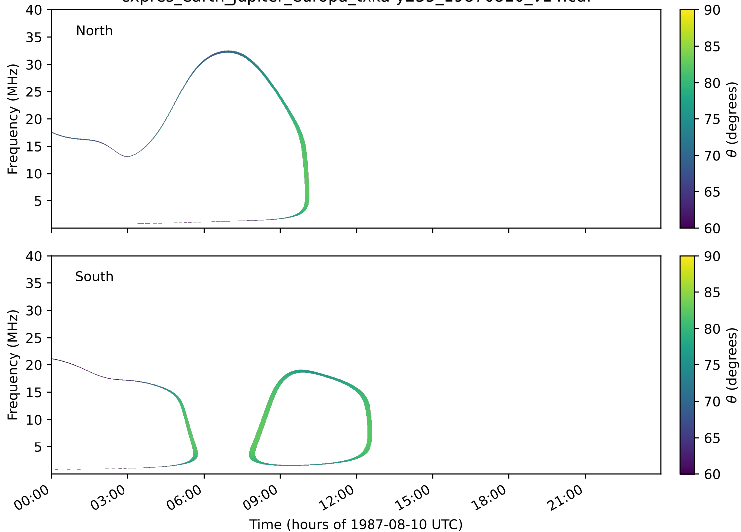
expres_earth_jupiter_europa_txka-y235_19870810_v14.cdf
