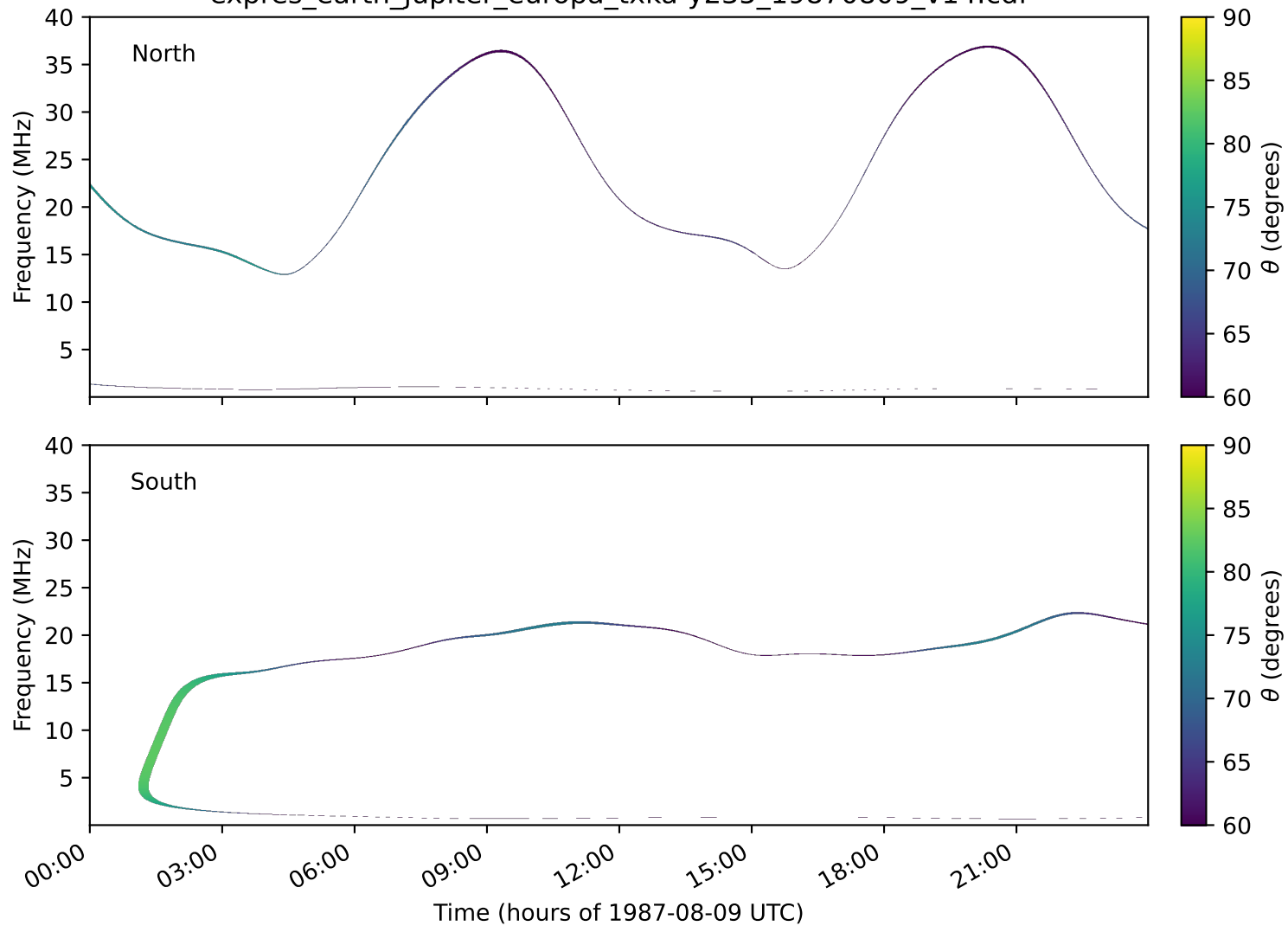
expres_earth_jupiter_europa_txka-y235_19870809_v14.cdf
