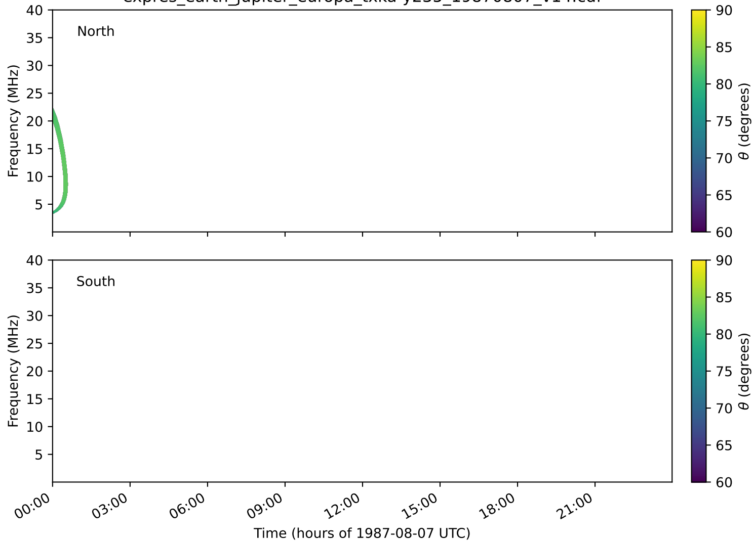
expres_earth_jupiter_europa_txka-y235_19870807_v14.cdf
