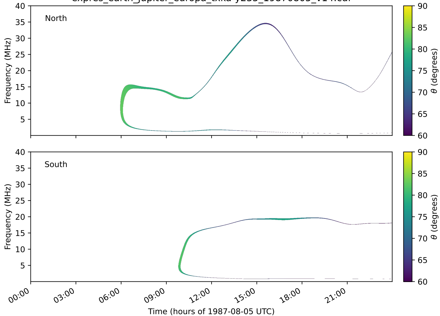
expres_earth_jupiter_europa_txka-y235_19870805_v14.cdf
