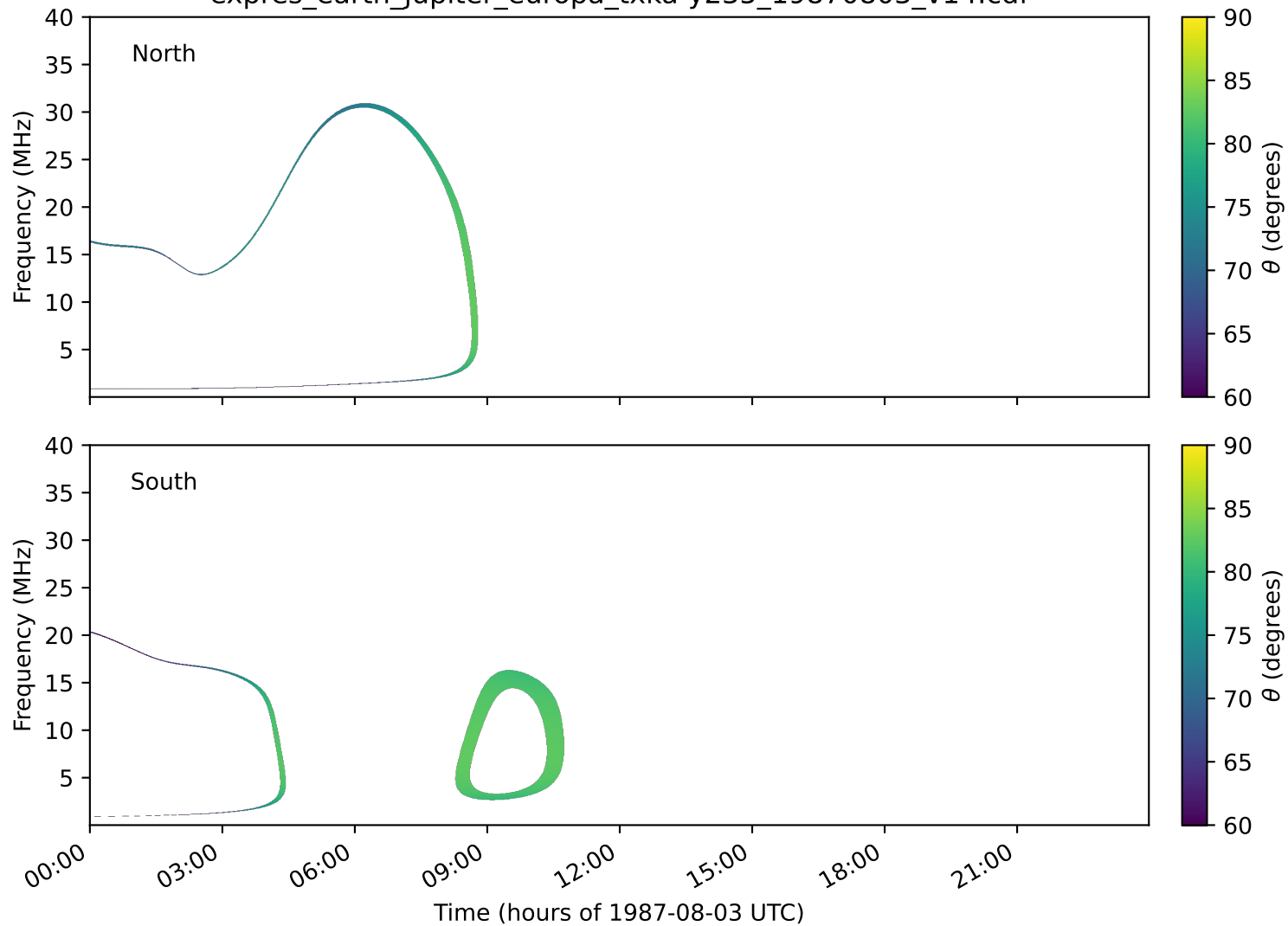
expres_earth_jupiter_europa_txka-y235_19870803_v14.cdf
