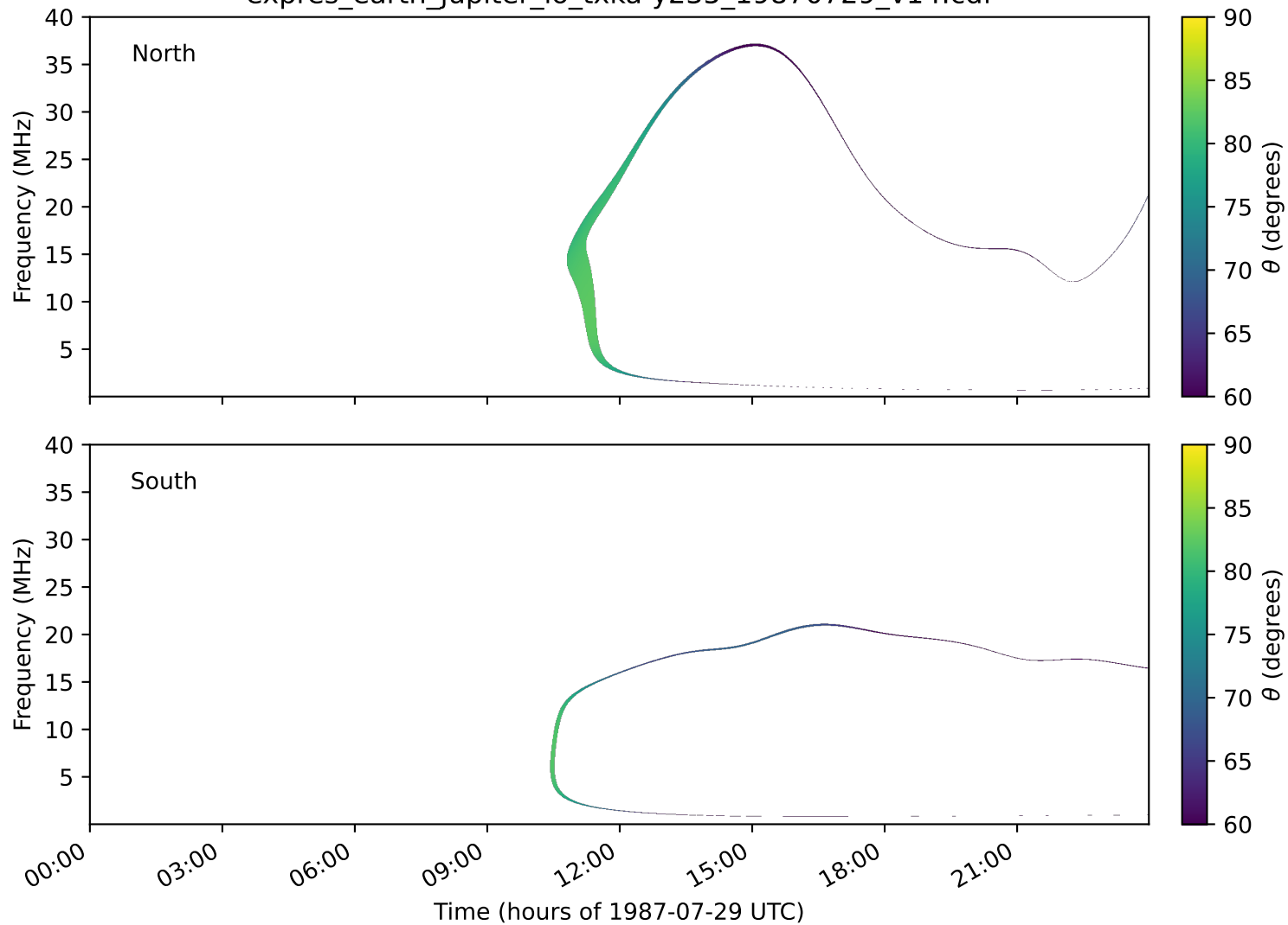
expres_earth_jupiter_io_txka-y235_19870729_v14.cdf
