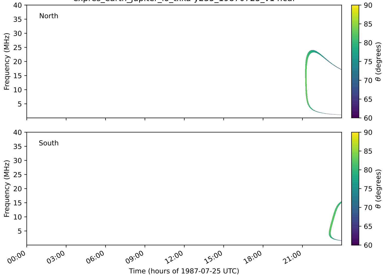
expres_earth_jupiter_io_txka-y235_19870725_v14.cdf
