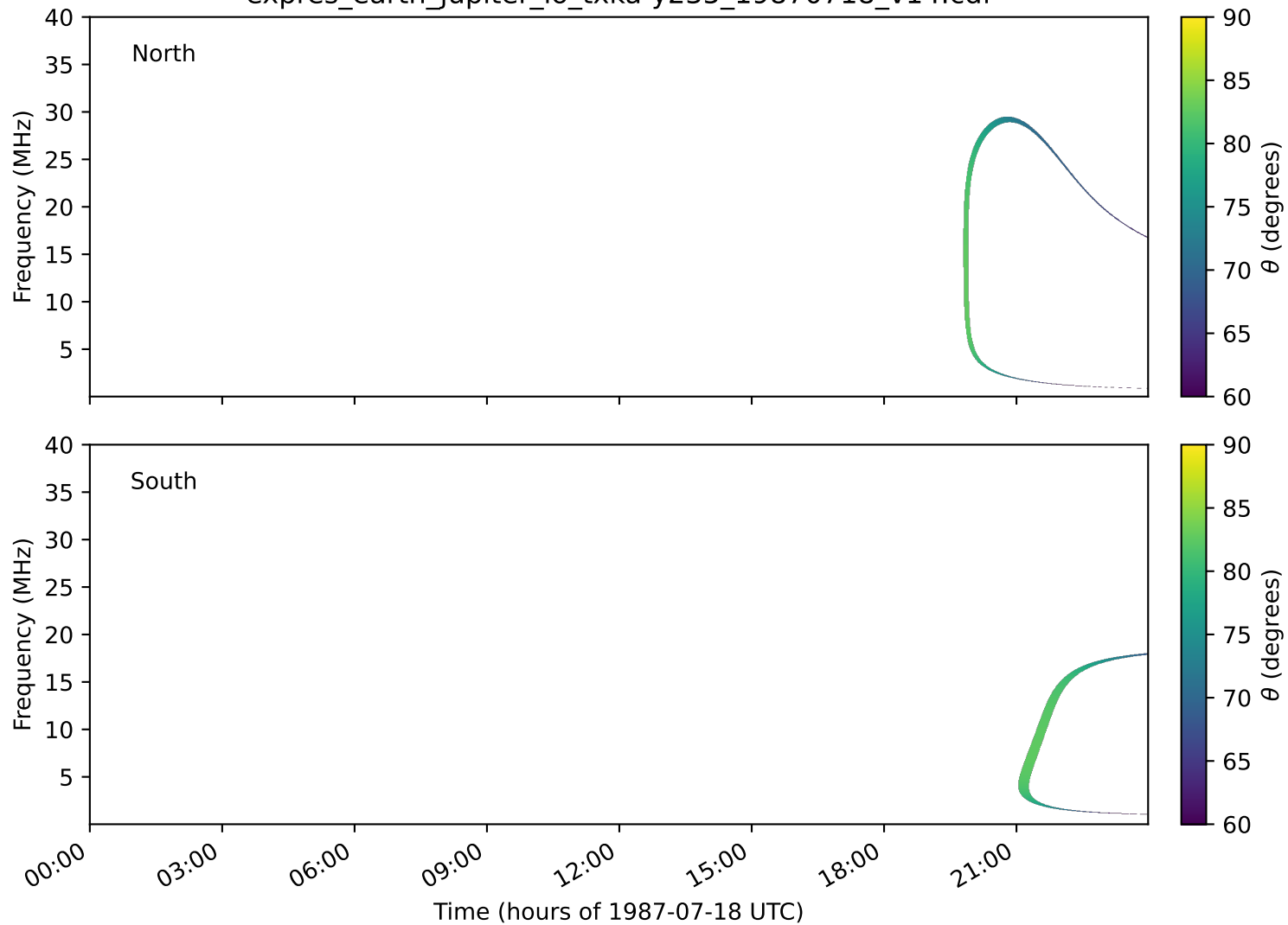
expres_earth_jupiter_io_txka-y235_19870718_v14.cdf
