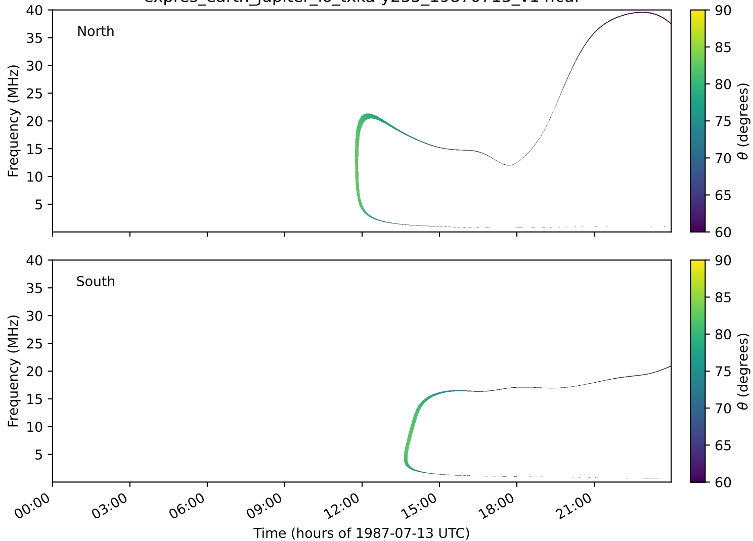
expres_earth_jupiter_io_txka-y235_19870713_v14.cdf
