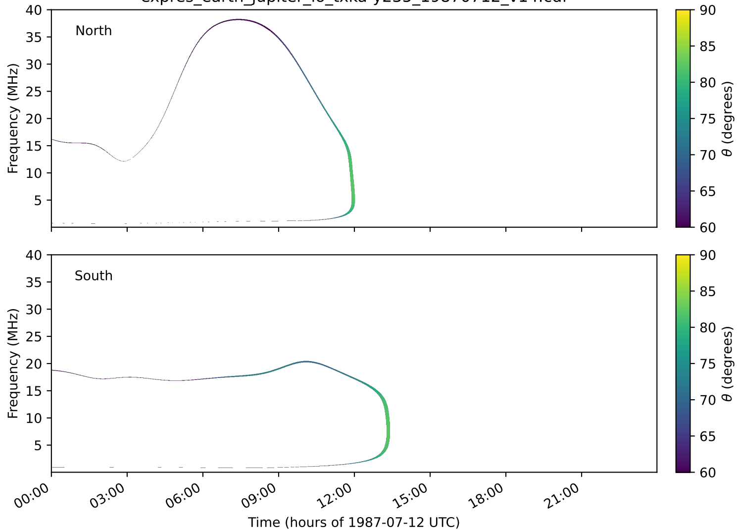
expres_earth_jupiter_io_txka-y235_19870712_v14.cdf
