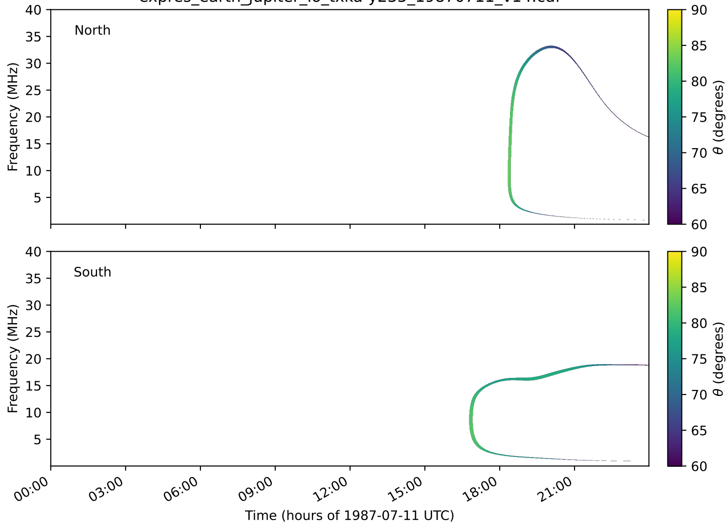
expres_earth_jupiter_io_txka-y235_19870711_v14.cdf
