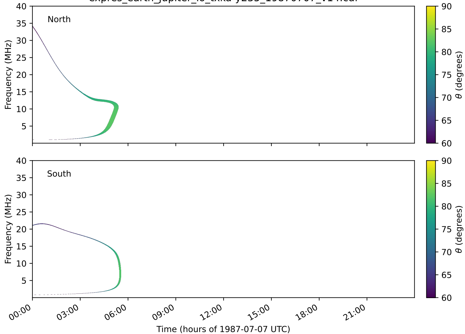
expres_earth_jupiter_io_txka-y235_19870707_v14.cdf
