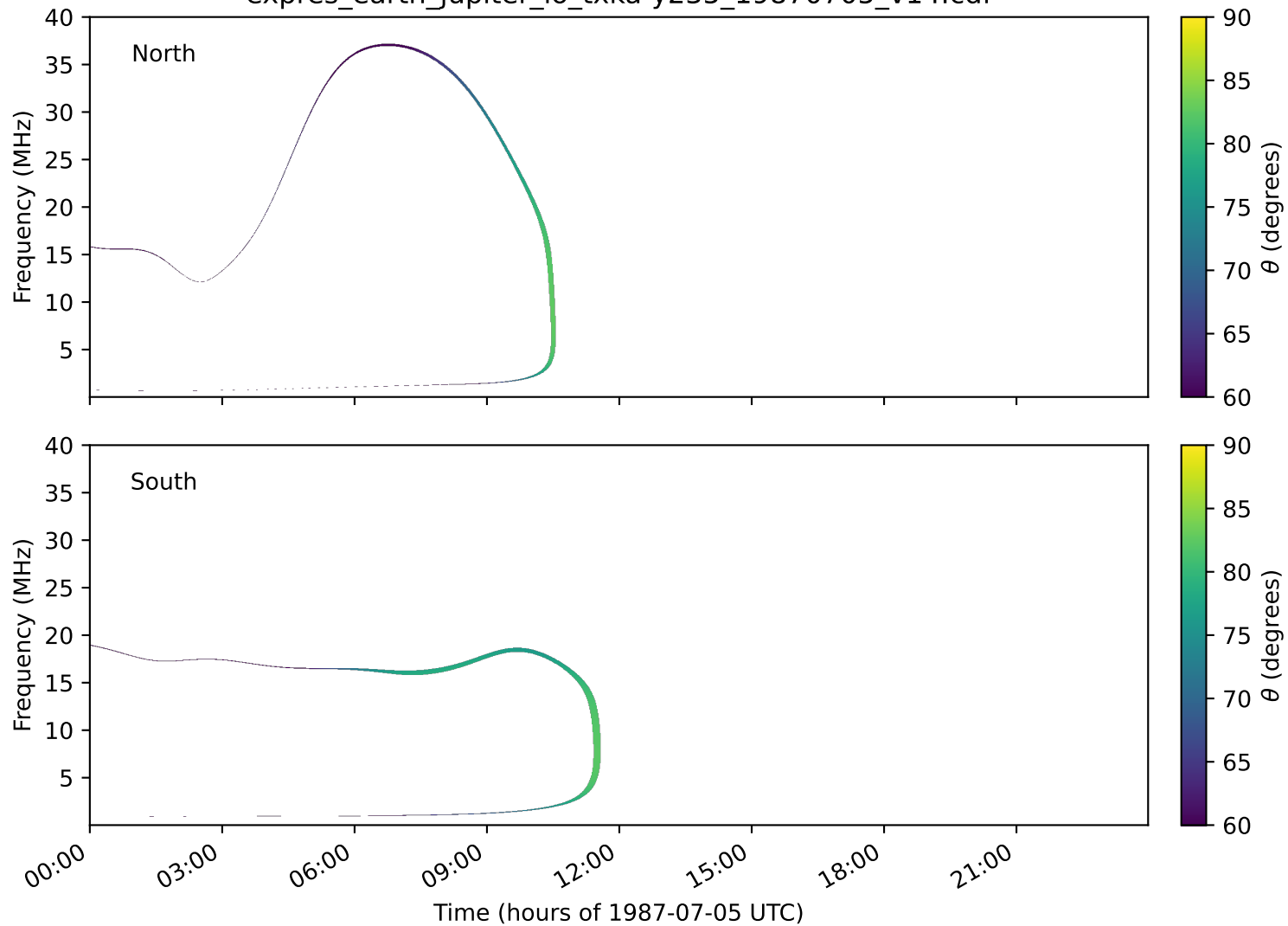
expres_earth_jupiter_io_txka-y235_19870705_v14.cdf
