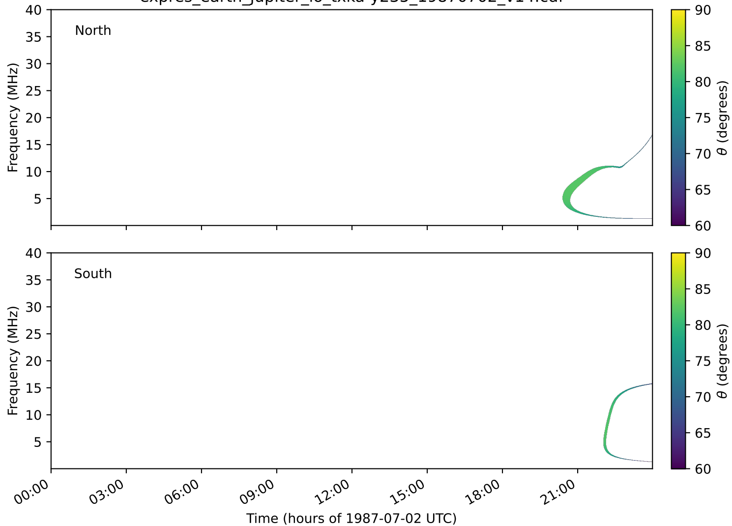
expres_earth_jupiter_io_txka-y235_19870702_v14.cdf
