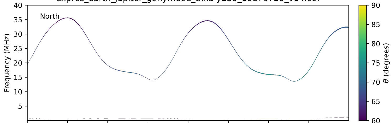
expres_earth_jupiter_ganymede_txka-y235_19870725_v14.cdf
