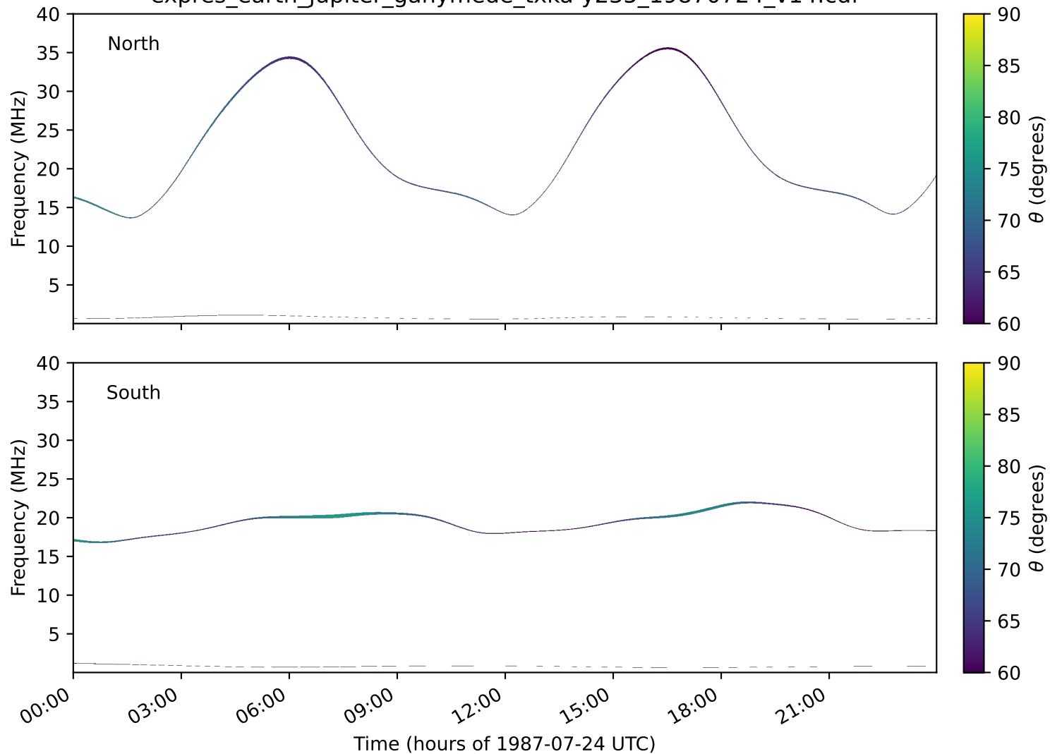
expres_earth_jupiter_ganymede_txka-y235_19870724_v14.cdf
