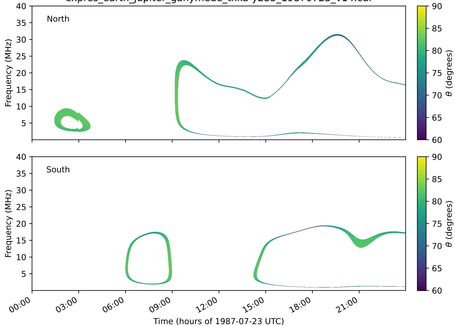
expres_earth_jupiter_ganymede_txka-y235_19870723_v14.cdf
