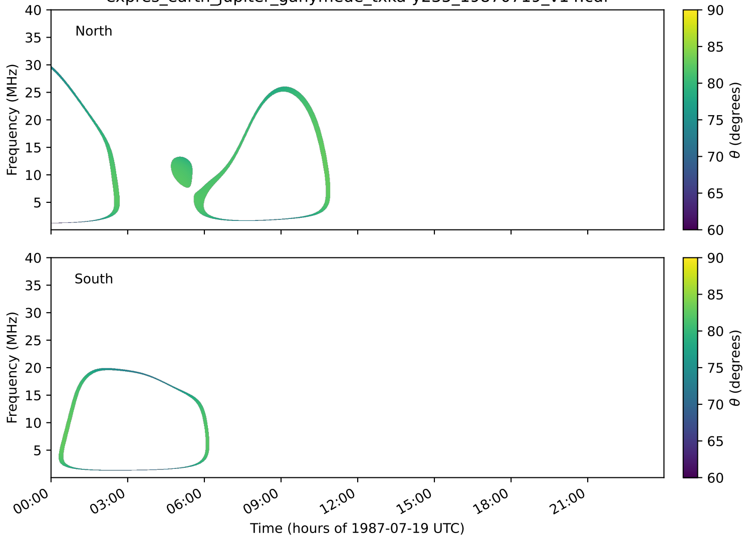
expres_earth_jupiter_ganymede_txka-y235_19870719_v14.cdf
