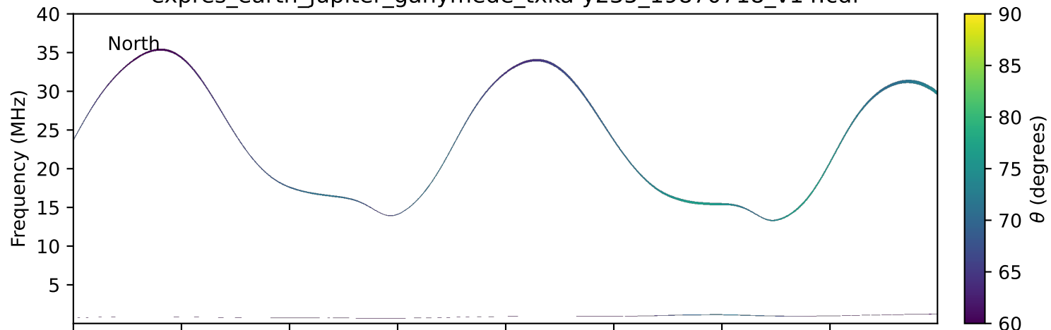
expres_earth_jupiter_ganymede_txka-y235_19870718_v14.cdf
