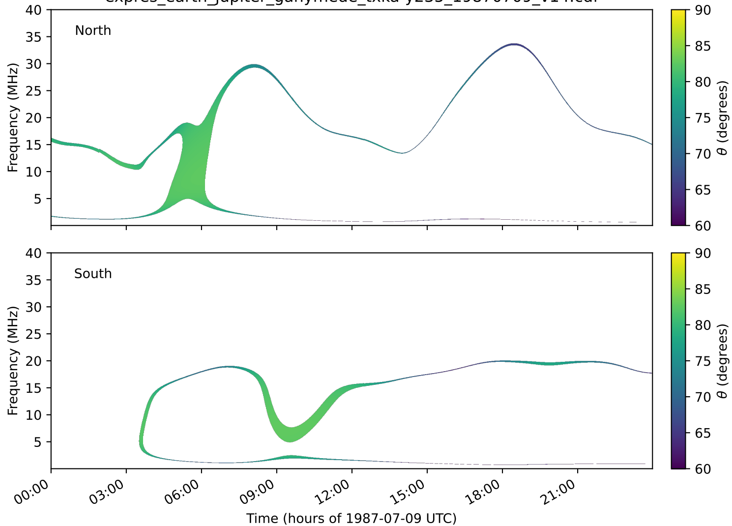
expres_earth_jupiter_ganymede_txka-y235_19870709_v14.cdf
