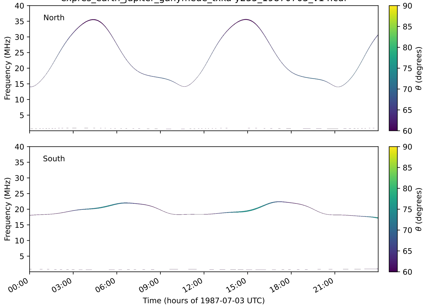
expres_earth_jupiter_ganymede_txka-y235_19870703_v14.cdf
