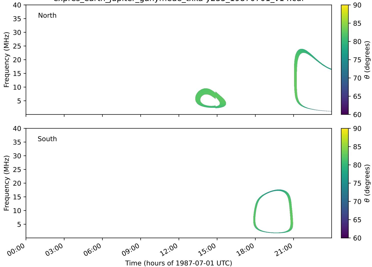
expres_earth_jupiter_ganymede_txka-y235_19870701_v14.cdf
