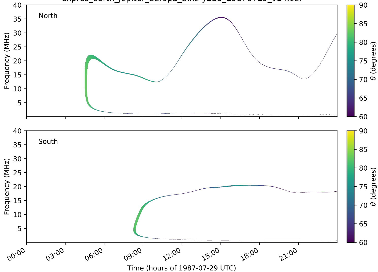
expres_earth_jupiter_europa_txka-y235_19870729_v14.cdf
