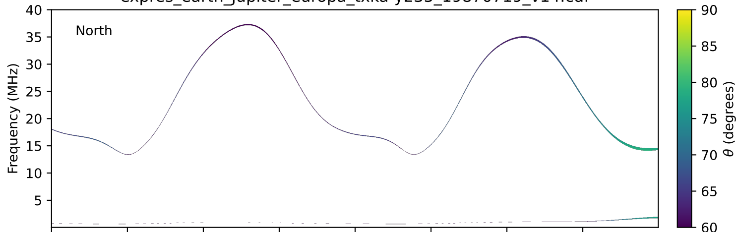
expres_earth_jupiter_europa_txka-y235_19870719_v14.cdf
