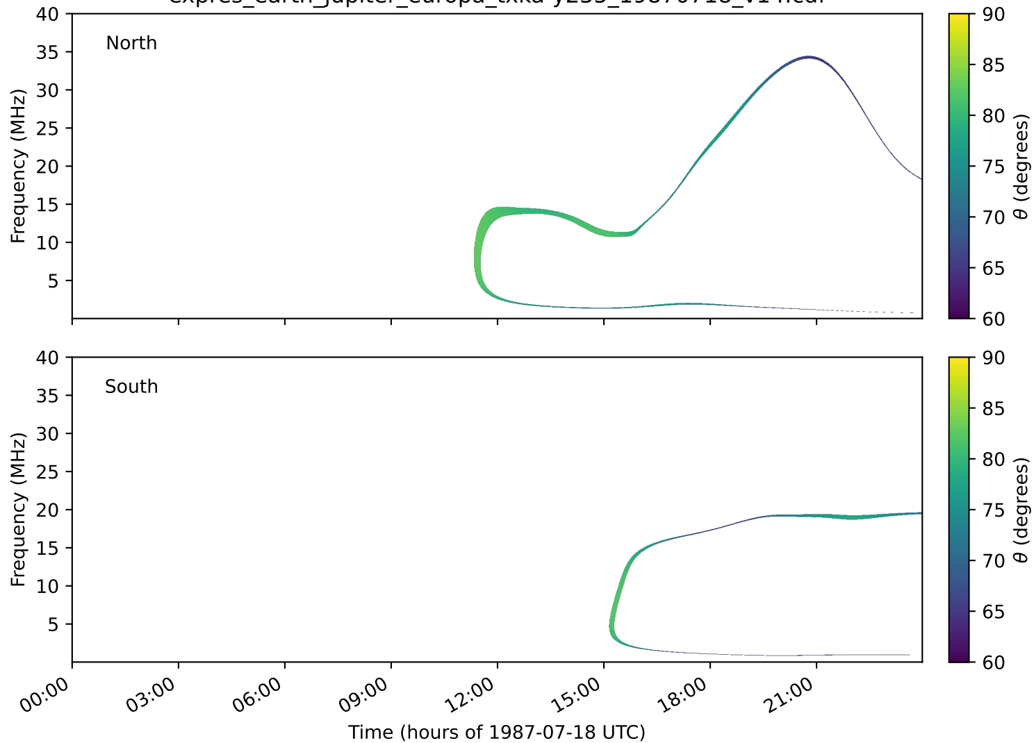
expres_earth_jupiter_europa_txka-y235_19870718_v14.cdf
