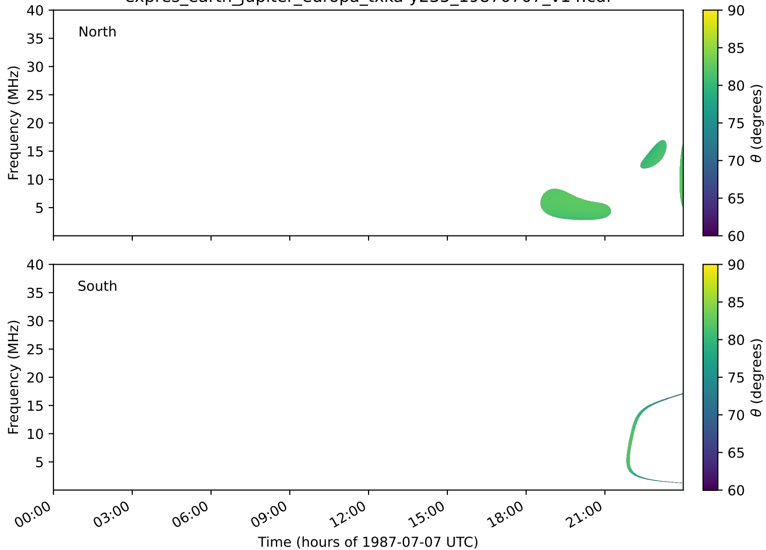
expres_earth_jupiter_europa_txka-y235_19870707_v14.cdf
