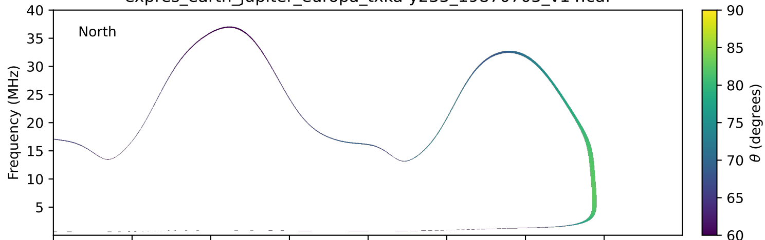
expres_earth_jupiter_europa_txka-y235_19870705_v14.cdf
