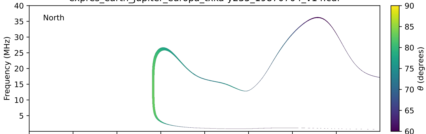
expres_earth_jupiter_europa_txka-y235_19870704_v14.cdf
