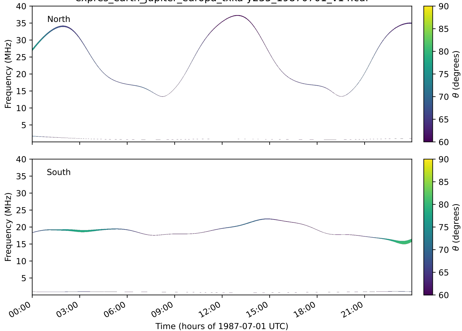
expres_earth_jupiter_europa_txka-y235_19870701_v14.cdf
