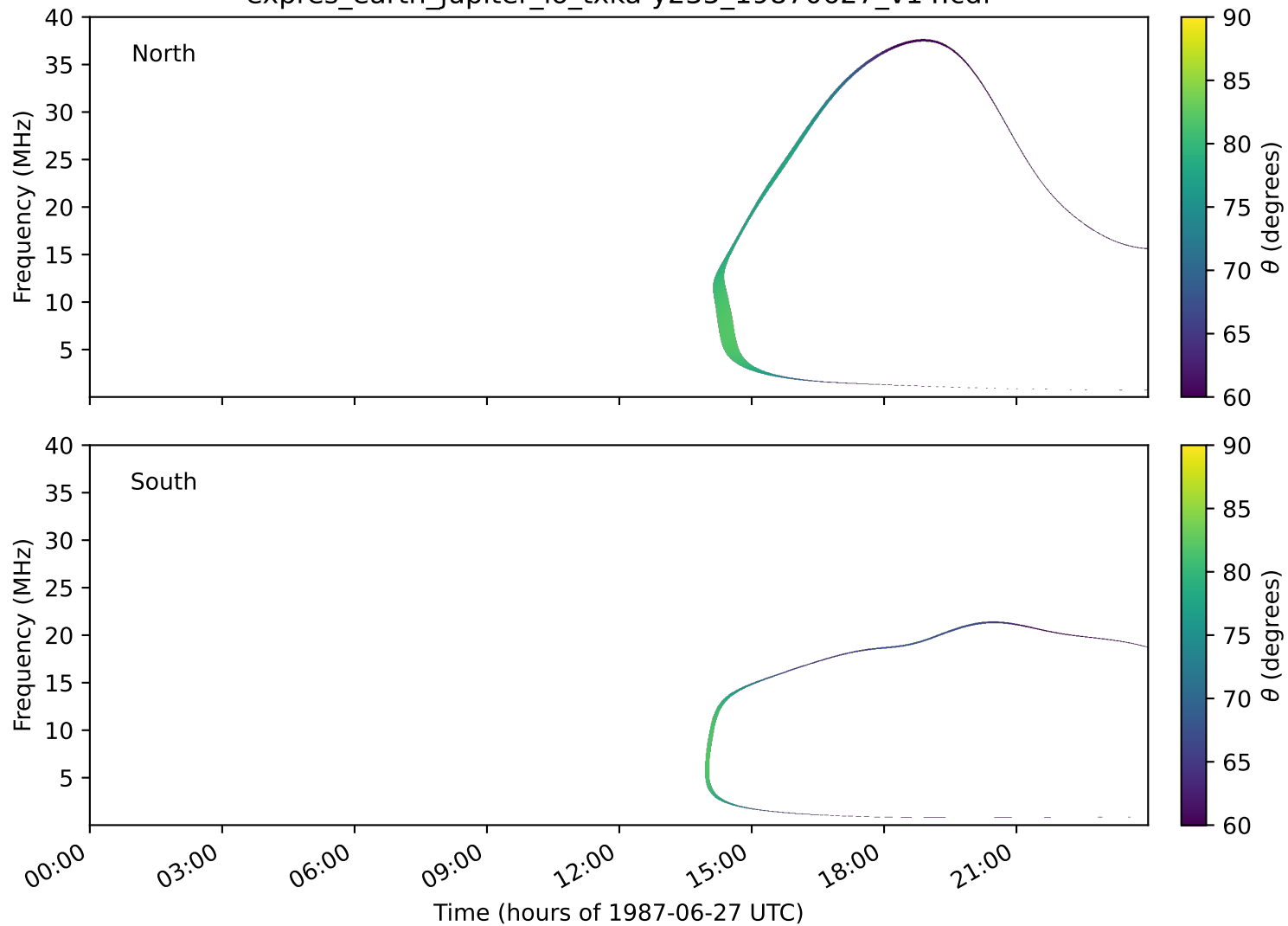
expres_earth_jupiter_io_txka-y235_19870627_v14.cdf
