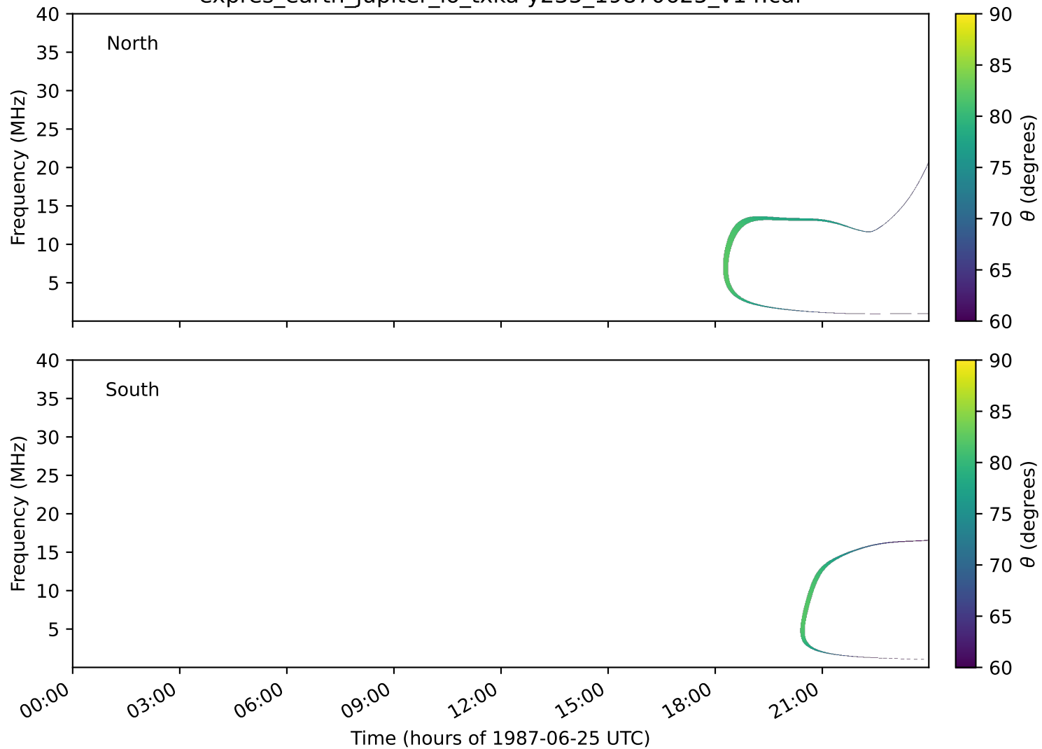
expres_earth_jupiter_io_txka-y235_19870625_v14.cdf
