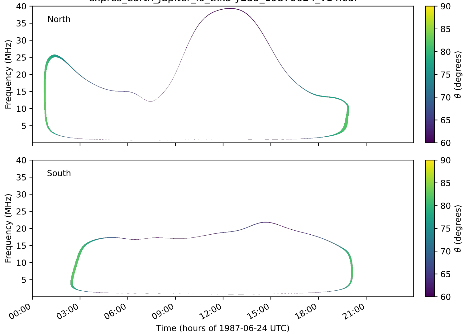
expres_earth_jupiter_io_txka-y235_19870624_v14.cdf
