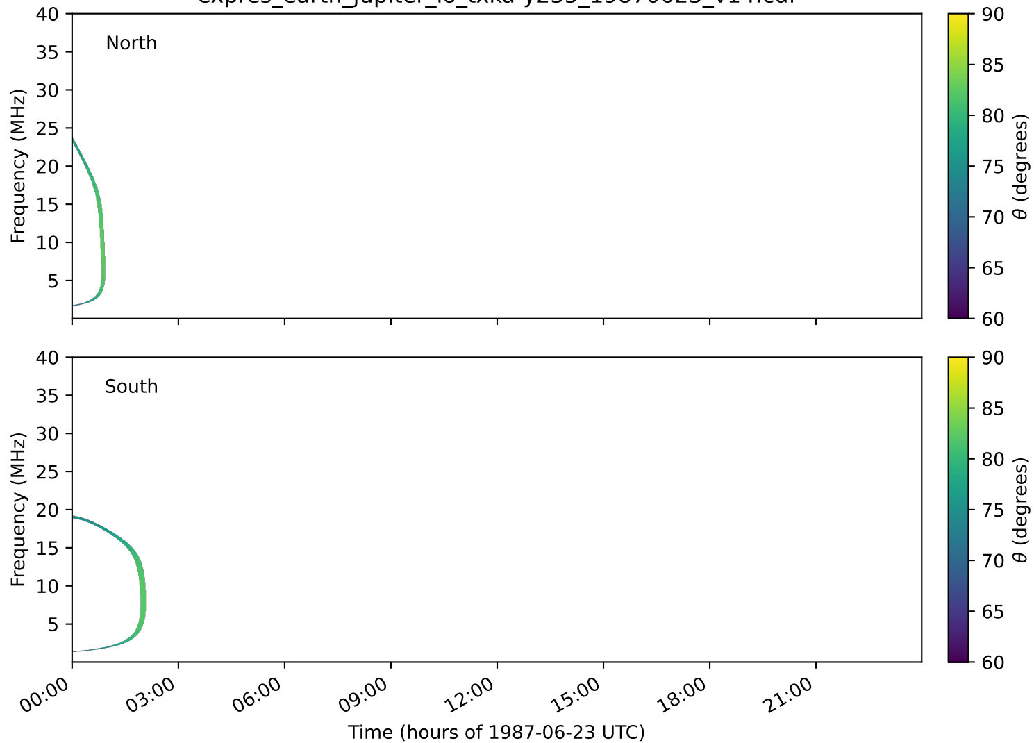
expres_earth_jupiter_io_txka-y235_19870623_v14.cdf
