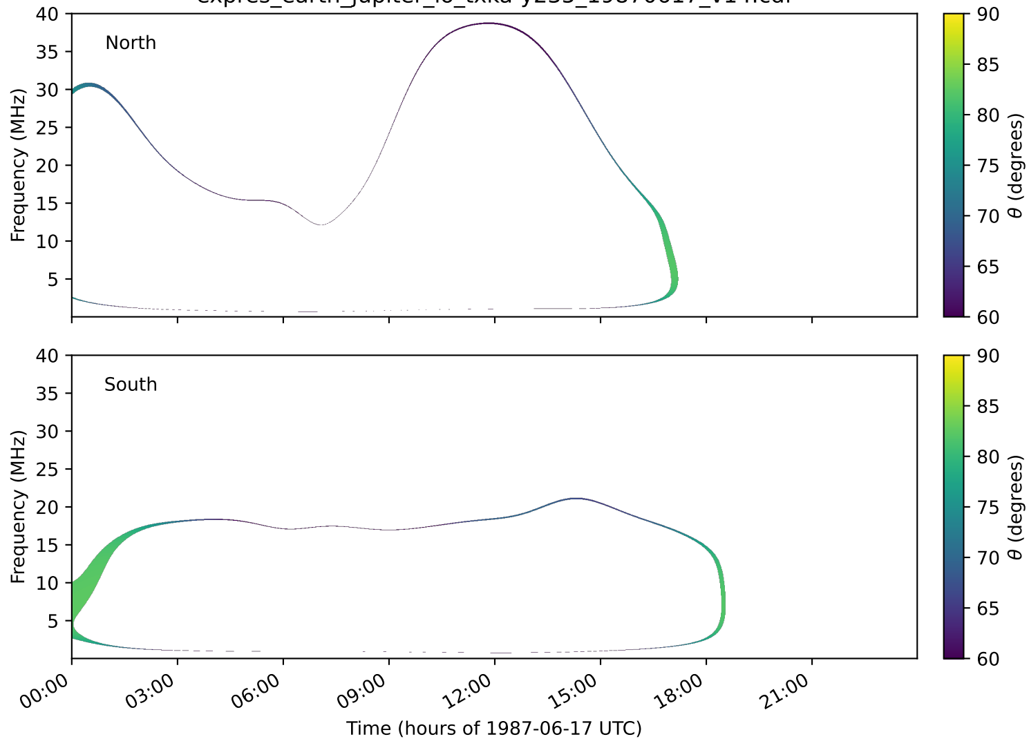
expres_earth_jupiter_io_txka-y235_19870617_v14.cdf
