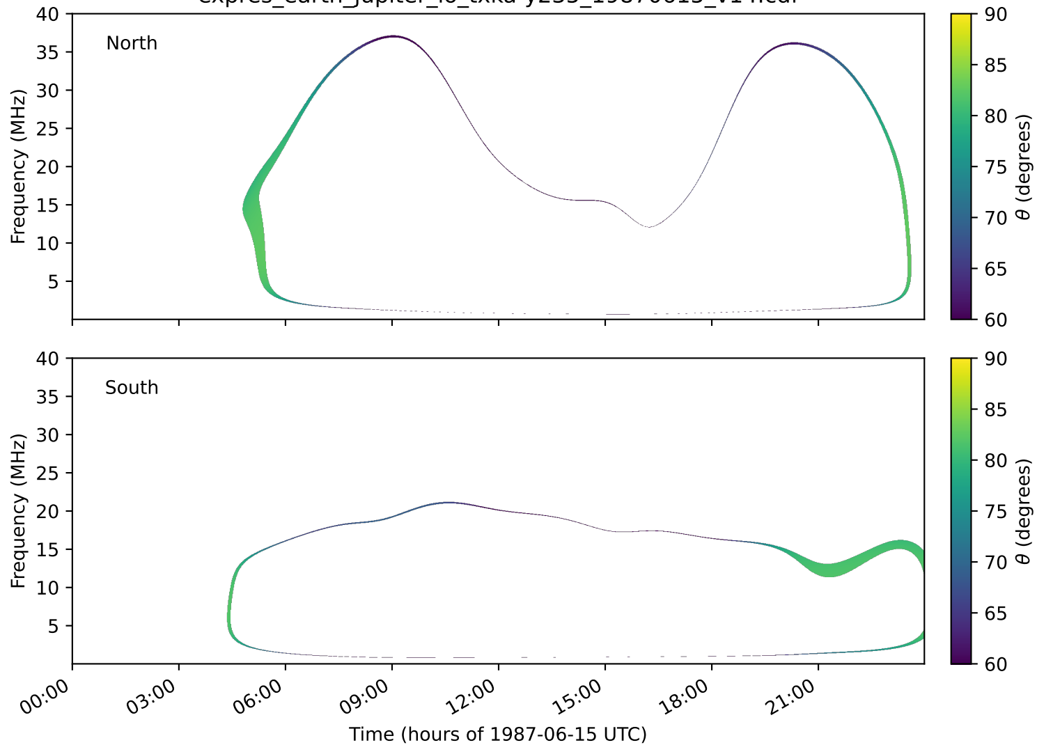
expres_earth_jupiter_io_txka-y235_19870615_v14.cdf
